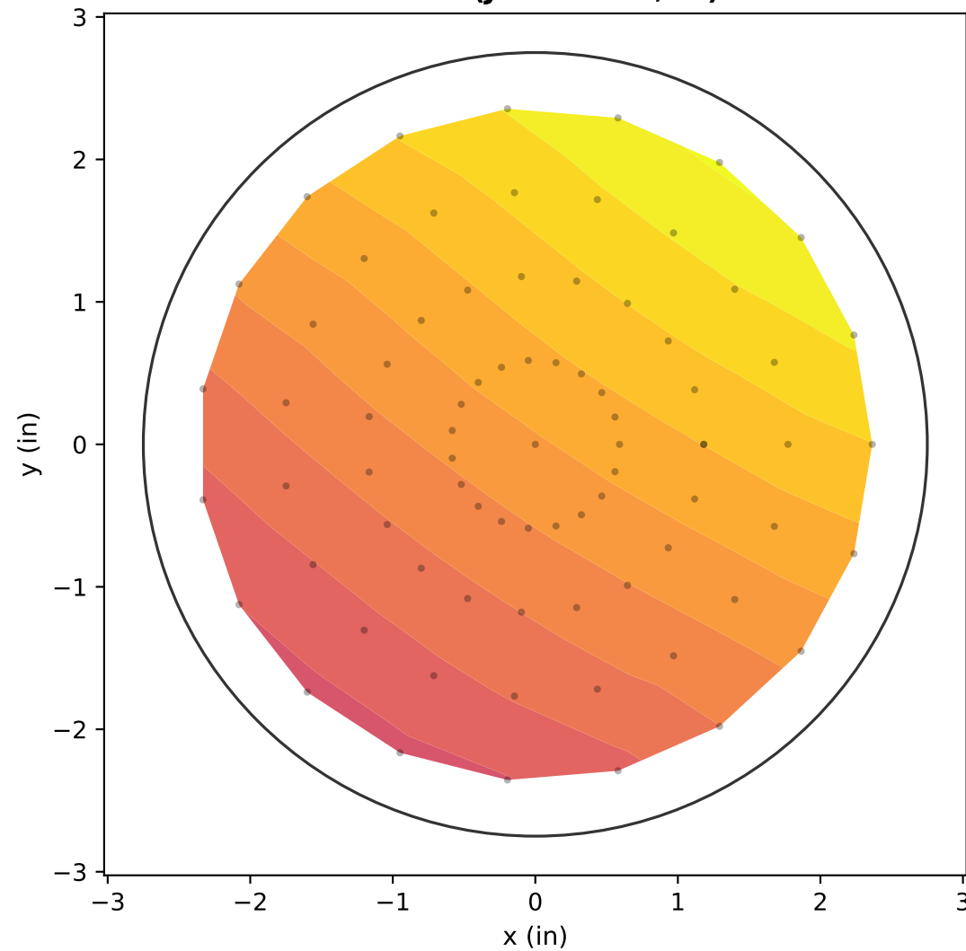
Slice 3 ( J=66.039 \text{ A/in}^2 )
