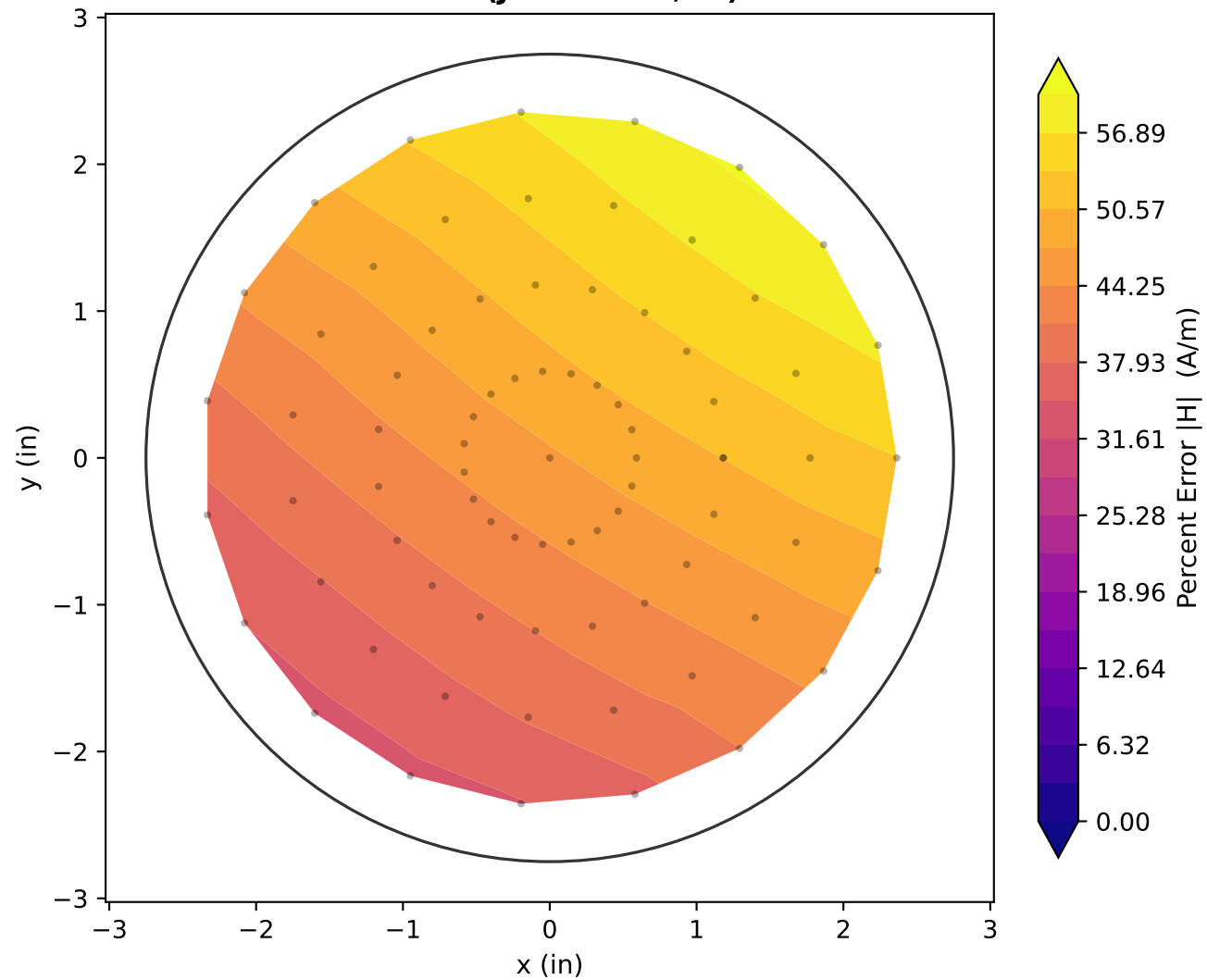
Slice 3 ( J=66.039 \text{ A/in}^2 )
